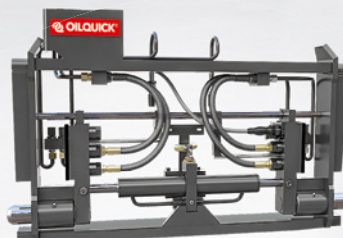
OILQUICK QUICK COUPLER QQT 300i
